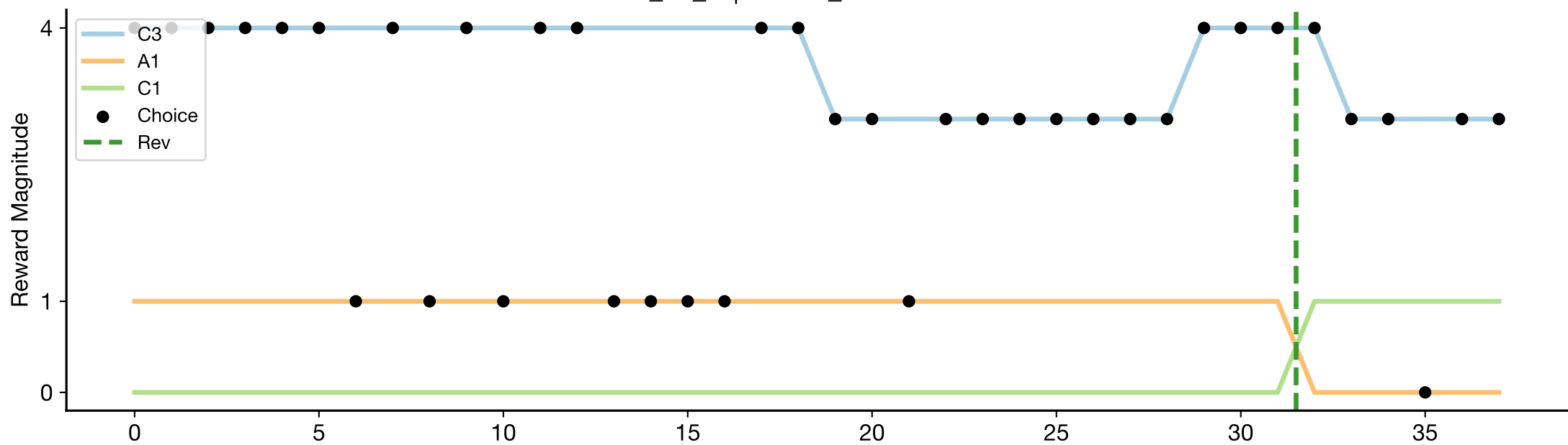
MY_72_N | ses-46_date-20260228
